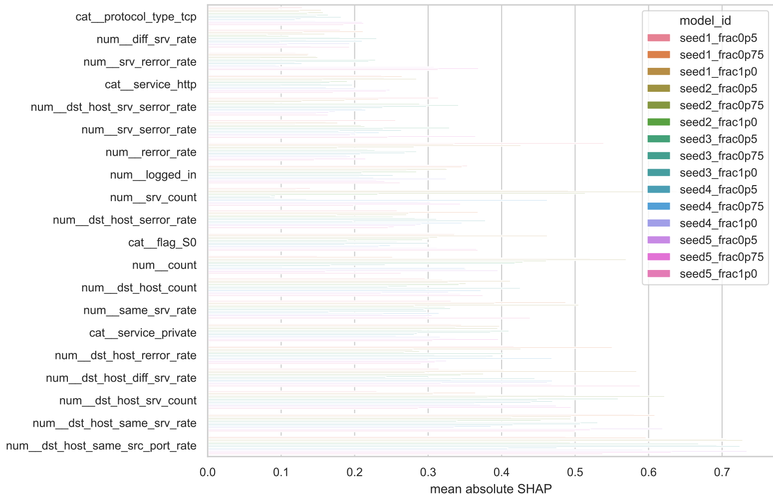
Top SHAP Features: attack
